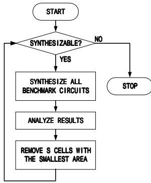
Fig. 1 Flowchart of library compacting algorithm.
