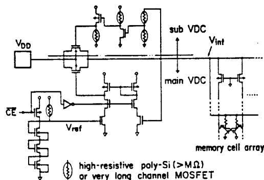
Fig. 2 Circuit diagram.
