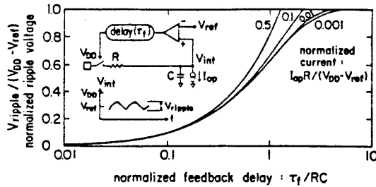
Fig. 10 Ripple voltage vs. feedback delay.
