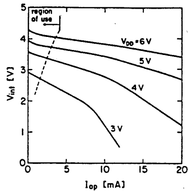
Fig. 5 Measured current supply characteristics.
