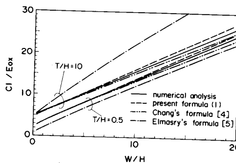
Fig. 2. Calculated wiring capacitance by various formulas.
